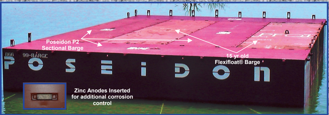
15 yr old Flexifloat® Barge
