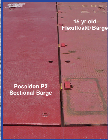
Zinc Anodes Inserted for additional corrosion control
